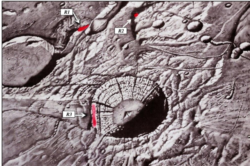
Figure 1. Patricia Bridges rendition of the TLP observed by James Greenacre and Edward Barr on October 30, 1963. Image originally published in 'Lunar Color Phenomena: Technical Report No. 12', USAF Aeronautical Chart and Information Center, St Louis, MO, 1964 May.
